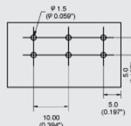
PCB Layout
