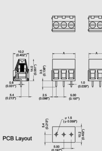
PCB Layout
